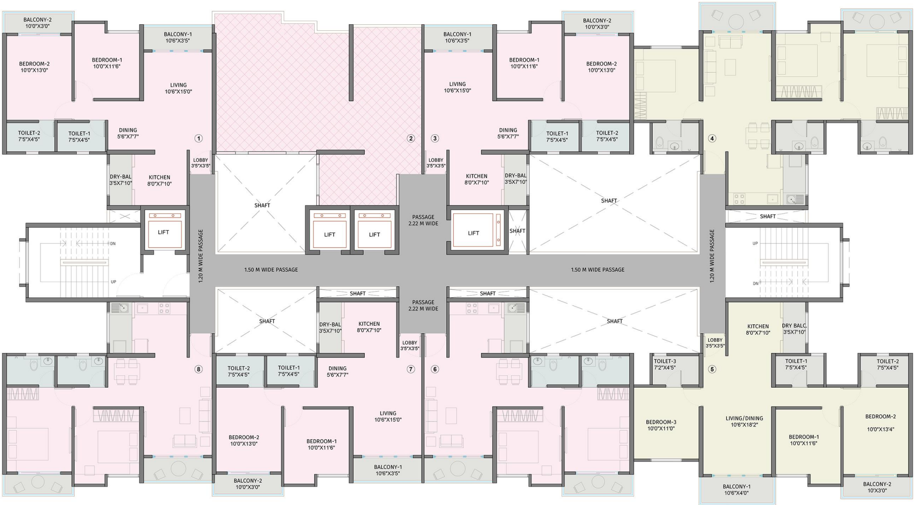
Tower 1 Refuge 7th,12th,17th & 22nd Floor Plan
